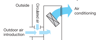
Return + Outdoor air mixed system
